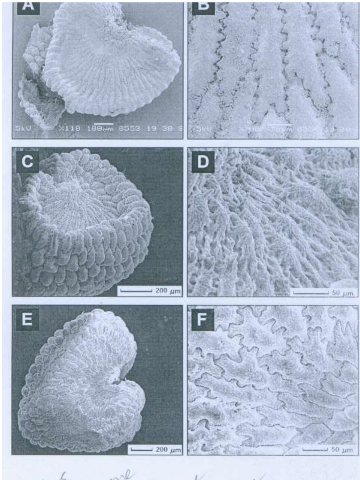
Fig.1. Scanning micrograph of Silene arenas : A, Seed; B, Seed surface; Silene brahuica : C, Seed; D, Seed surface; Silene citrian : E, Seed; F, Seed surface.
