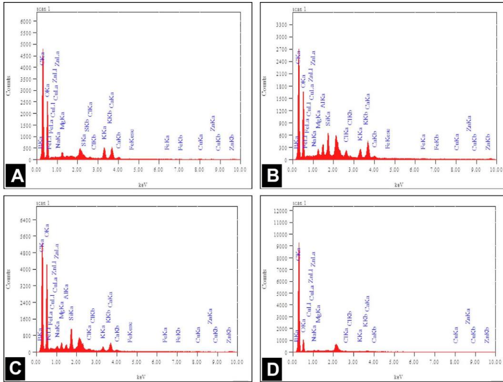
Fig. 1. Energy-dispersive X-ray spectroscopy (EDS) graphs showing leaf elemental composition. A , Cleome ariana ; B , C. brachycarpa ; C , C. dolichostyla ; D , C. karachiensis .
