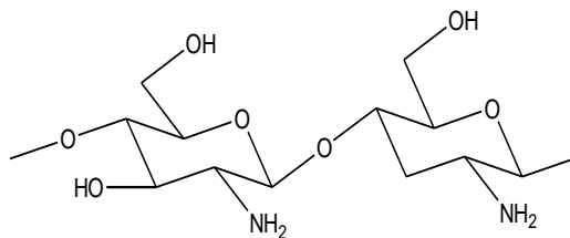
Fig 1: Chitosan structure
