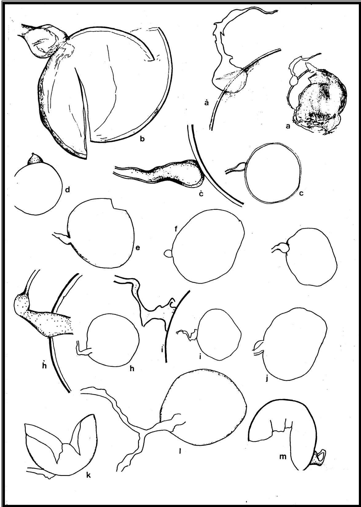
Fig.3. Spores formed freely in soil aggregates
