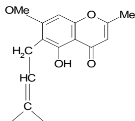
peucenin-7-methyl ether
