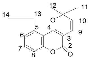
17-methylbothrioclinin
