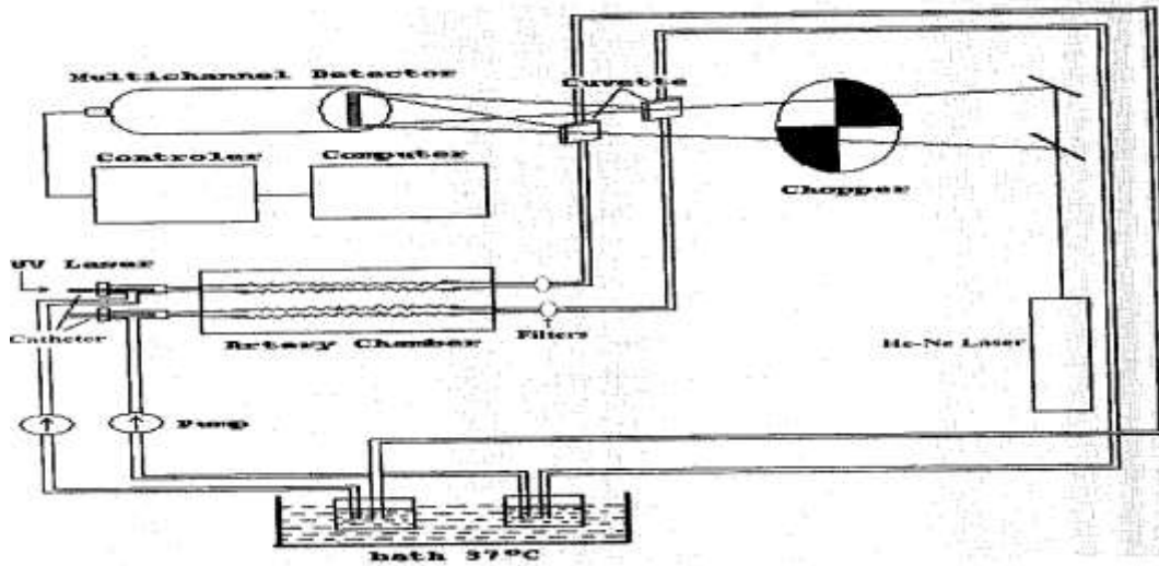
Fig. 1. Dual Organ Chamber Experiment Set Up. The He-Ne laser beam is split by a beam chopper to enter the cuvettes and displayed the laser light scattering on the diode array at 1°5'.
