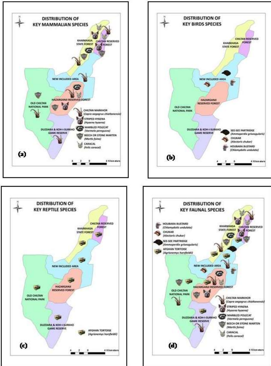
Fig. 5. Distribution of Selected Key (a). Mammalian Species, (b). Birds Species, (c). Reptile Species and (d).all funal Species.
