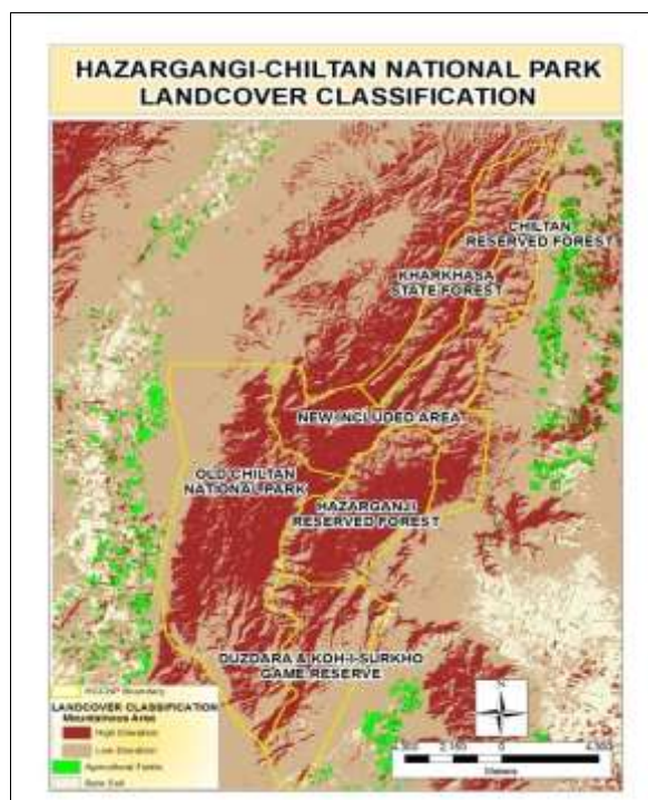
Fig. 3. Hazarganji-Chiltan National Park: Land Cover Classification.
