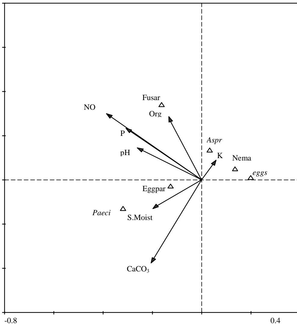
Fig. 1. CCA-ordination diagram of the sampling plots with biological ( \Delta ) and environmental variables (arrows); first axis is horizontal, second axis vertical. The biological variables including root-knot nematode and fungi. The fungi are: A. spp. = Aspergillus spp, Paeci = Paecilomyces lilacinus , Fusar = Fusarium solani . And nema = nematode soil population, eggs = number of eggs, eggpar = egg parasitism.
