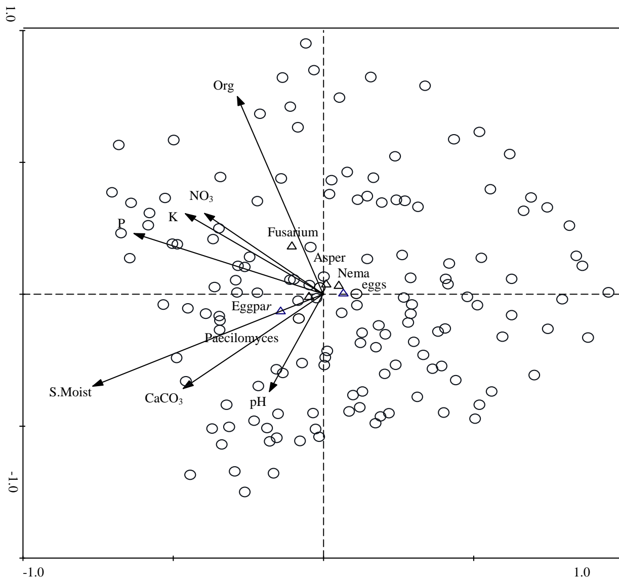
Fig. 2. Triplot from a CCA of the root-knot nematode and soil fungi of tomato egg plants. Environmental variables are represented by arrows, samples (quadrats) by small open circles, and species by triangle ( \Delta ). The species are listed by the initial letters of the genus and the specific epithet, they include: A. fumig. = Aspergillus spp., Paeci = Paecilomyces lilacinus , Fusar = Fusarium solani . And nema = nematode soil population, eggs = number of eggs, eggpar = egg parasitism.
