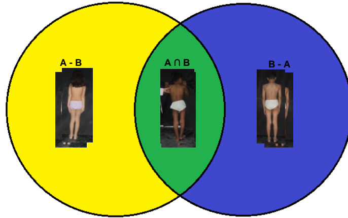
Fig. 9.Venn-diagrammatic representation of intersection and difference sets
